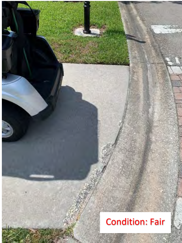
(248) Chipped Sidewalk
