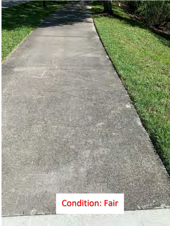
(235) Elevated Corners, Corner and Center Cracks
