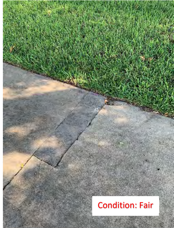
(64) Elevated Corner and Corner Crack (2)
