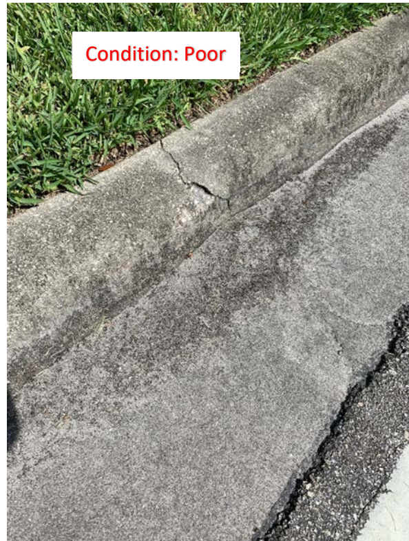
(1) Curb and Gutter Cracking (2)
