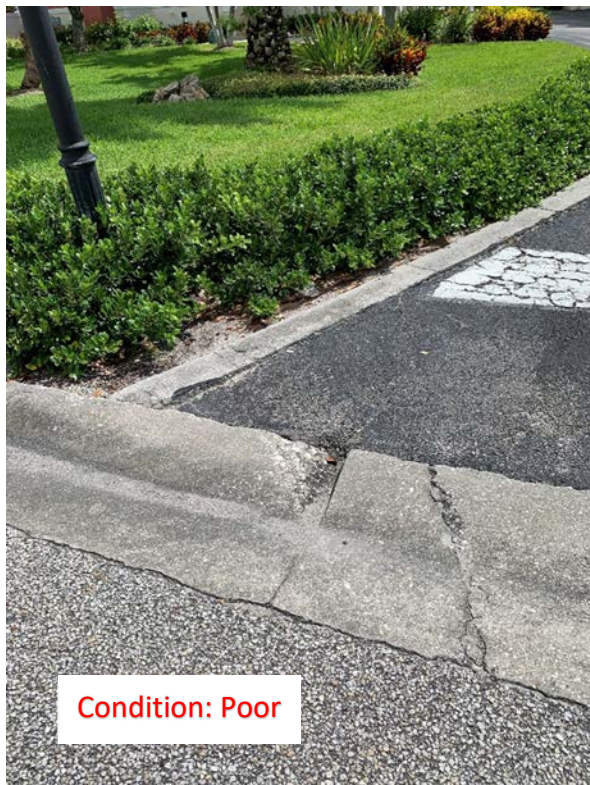
(7) Chipped Gutter
