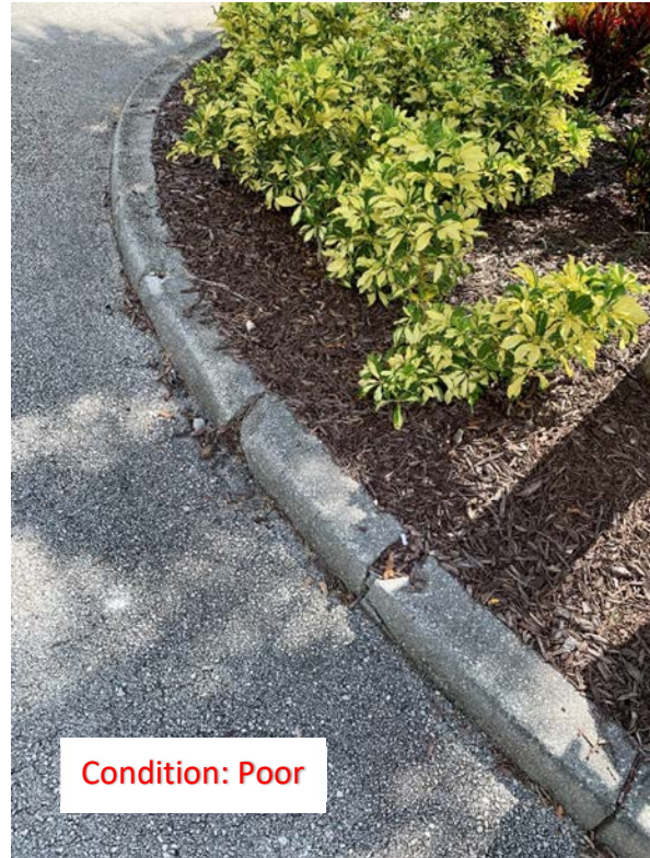
(3) Curb Cracking and Chipping (2)
